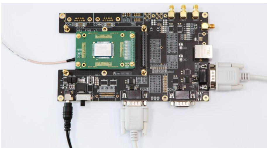
Figure 3-1 Connection
